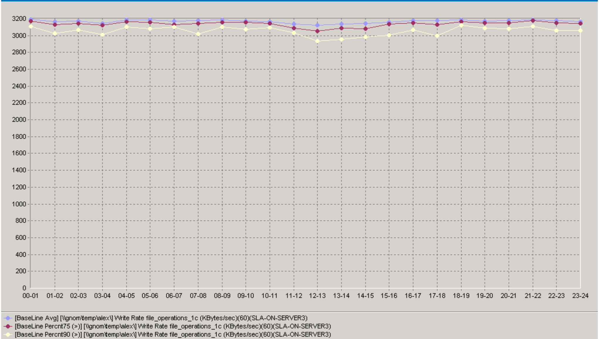
60 [\vgnom\temp\alex\] Write Rate file_operations_1c (KBytes/sec)
